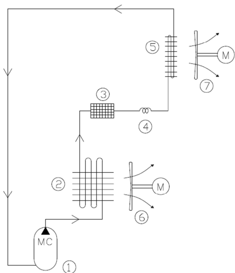
Process Chiller Working Principle
